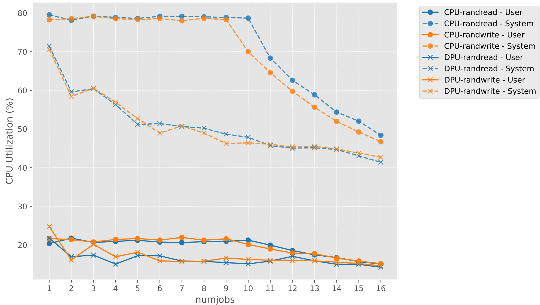
CPU Utilization vs numjobs
